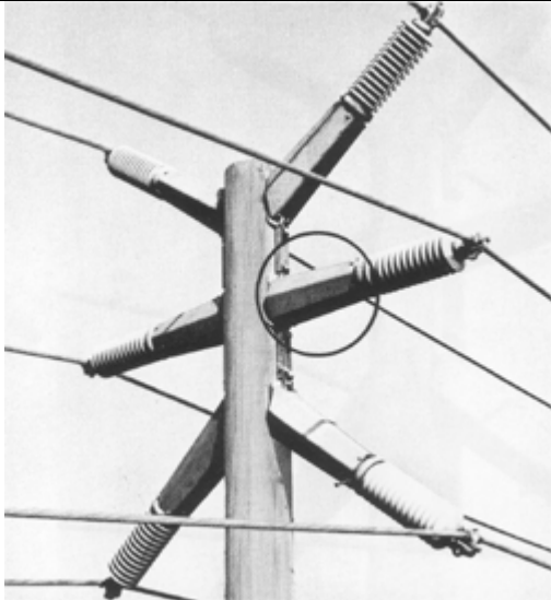
Heavy Duty Fail-Safe Extension Arms with Shroud
