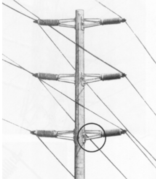
Heavy Duty Fail-Safe Extension Arms
