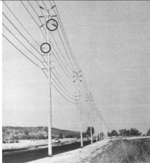
Combination Heavy Duty Light Duty Extension Arms
