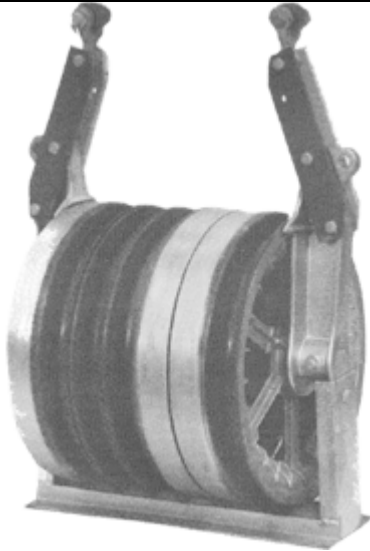
6103 Series Offset Traveler
