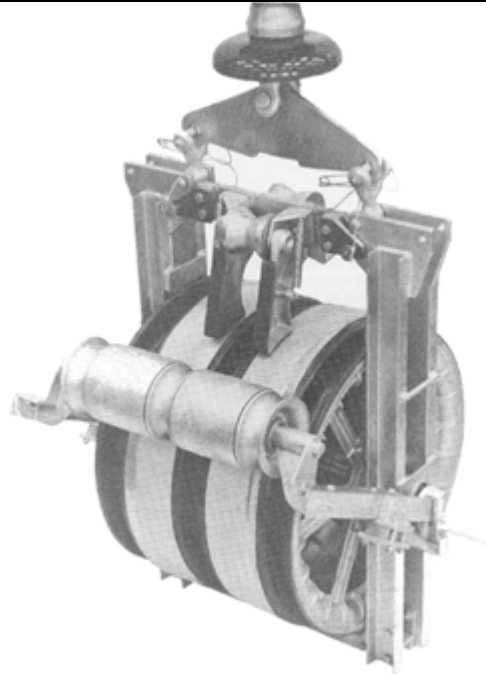
6650 Series Traveler with 6041 Automatic Uplift Roller and 6580 Traveler Ground
